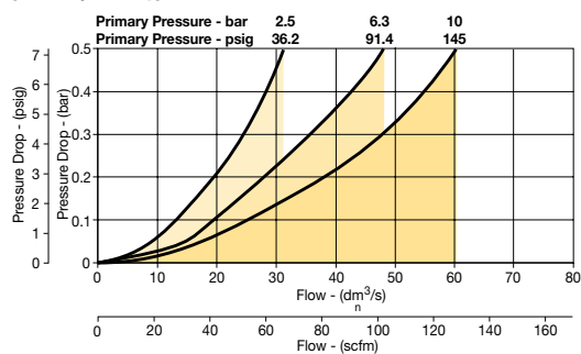
P32FB 1/2" Filter
