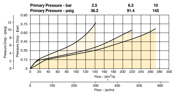
(1") Lubricator
