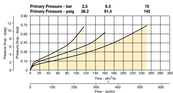
(3/4") Lubricator
