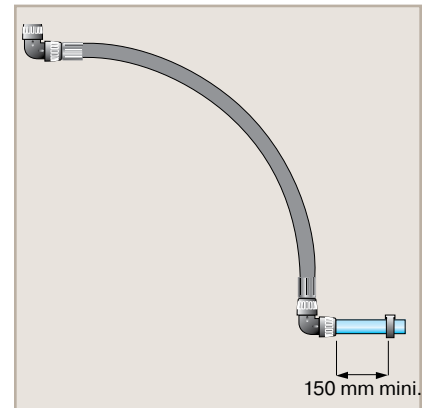
Obstacle bypass
